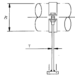
Variant A with bottom plate
