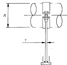
Variant A with bottom plate
