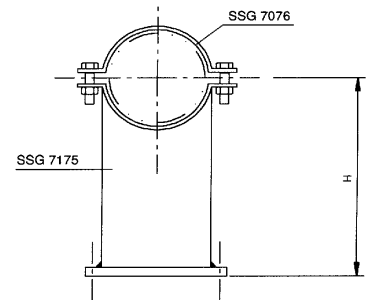
Variant A with bottom plate
